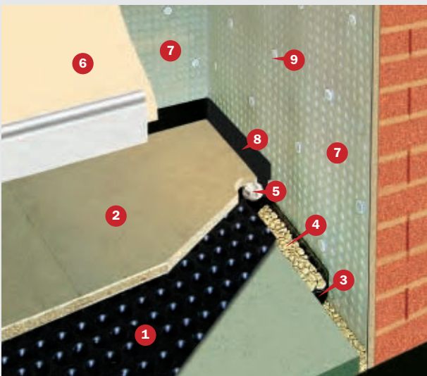
1) P20 Membrane 2) Chipboard 3) Aqua Channel 4) 20mm Stone 5) Jetting Eye 6) Plaster/Render 7) Plaster Base Membrane 8) Wall/Floor Junction 9) Plaster Plug
